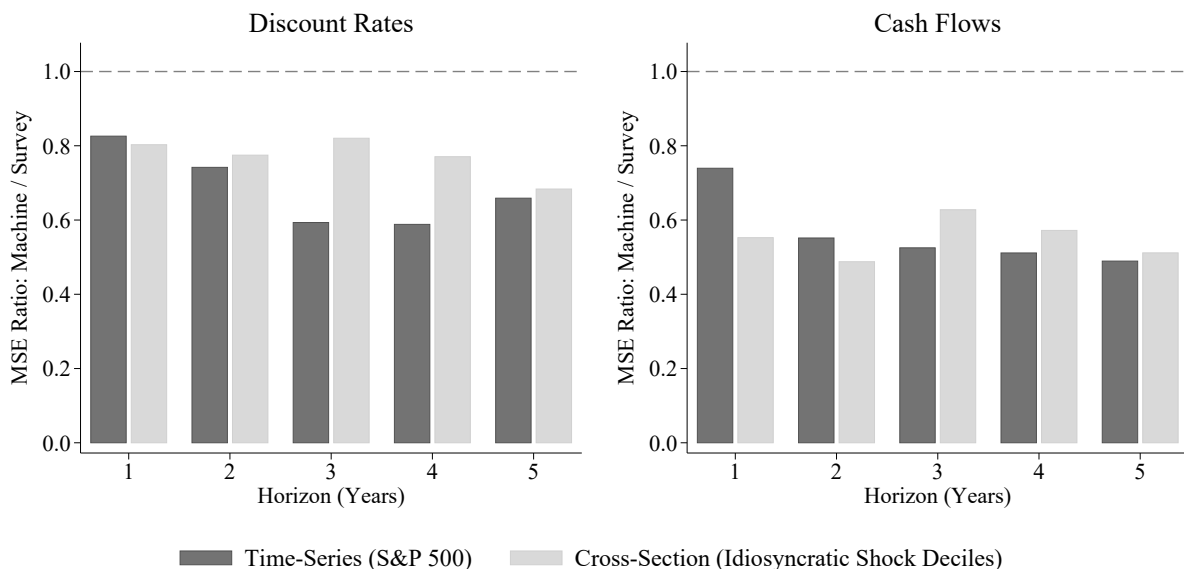
Figure 1: Accuracy of Machine Learning vs. Survey Forecasts
